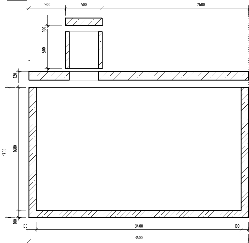
REZ 1-1 M1:25
